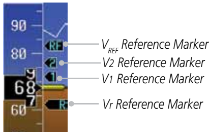
Figure 2-11 Alternate Reference Speeds
