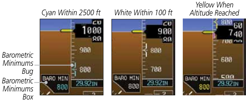
Figure 2-23 Barometric MDA/DH Alerting Visual Annunciations
