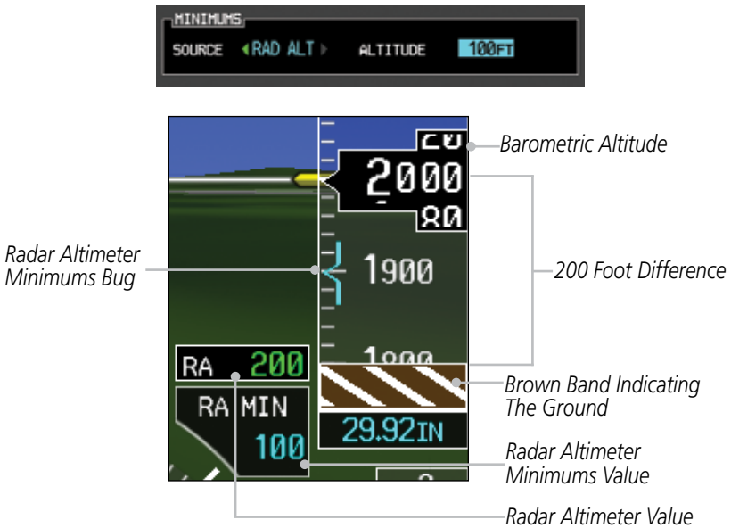
Figure 2-24 Minimums Values with a Radar Altimeter
