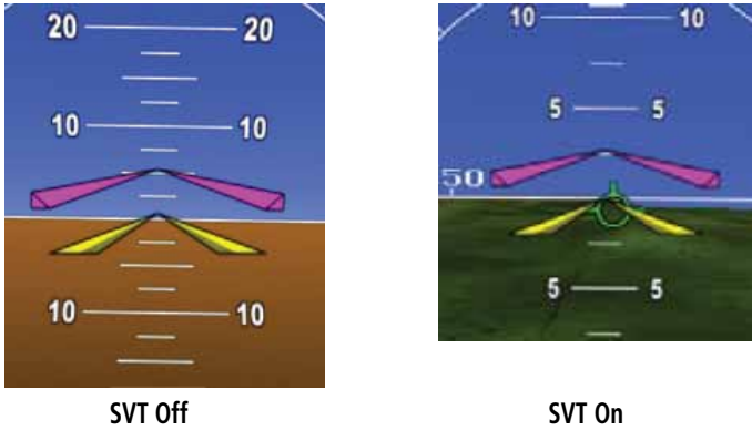
Figure 5-33 Flight Director Bars Showing Aircraft Pitch
