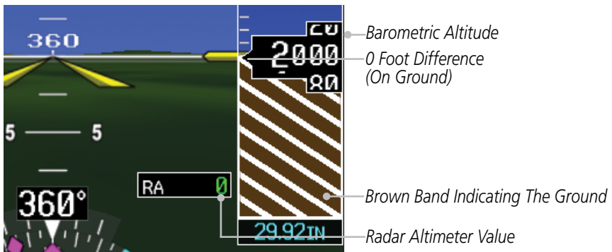
Figure 2-45 Radar Altimeter Display - 0 foot RA Altitude
