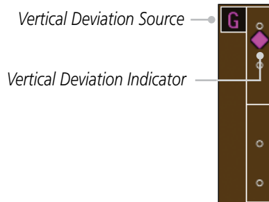
Figure 2-33 Vertical Deviation Indicator (GPS Source)
