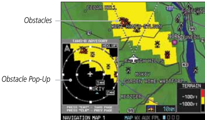
Figure 5-48 Obstacle Depiction on MFD
