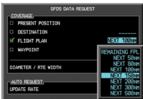
Figure 4-101 Flight Plan GFDS Data Request
