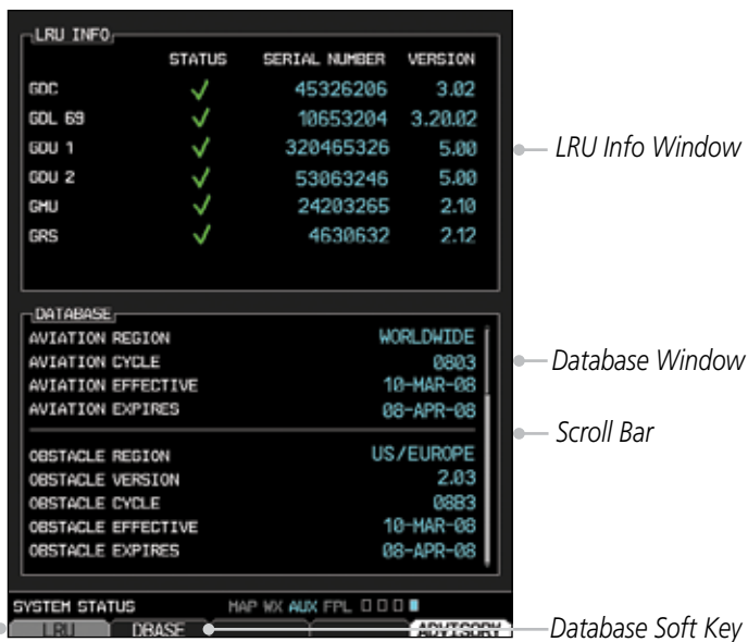
Figure 3-82 LRU and Database Information
