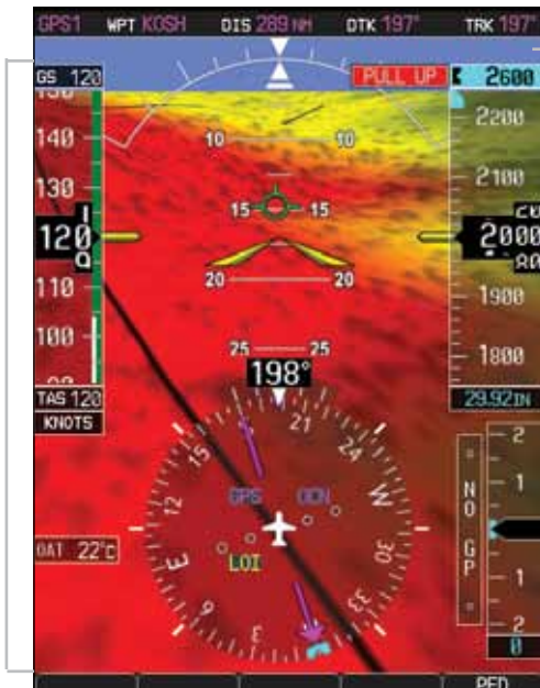
Figure 5-54 Blue Sky Bar with Full Display Terrain
