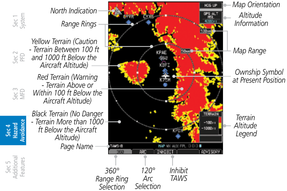
Figure 4-11 360° View on the TAWS Page
