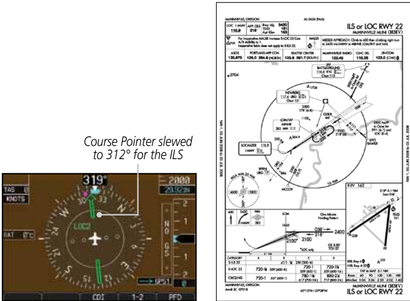
Figure 2-34 Auto-Slewing HSI with ILS Loaded and Shown with the Corresponding Approach Plate
