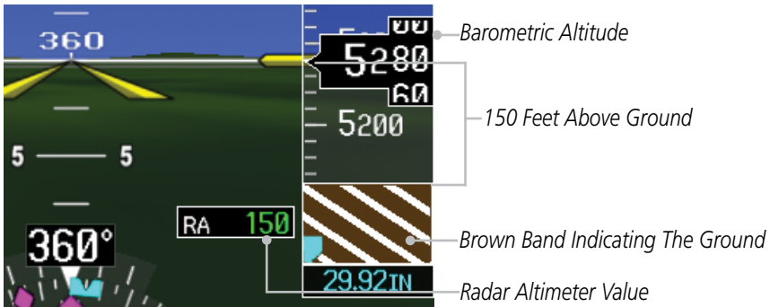
Figure 2-44 Radar Altimeter Display - 150 foot RA Altitude
