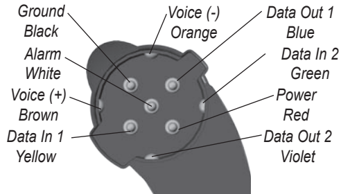
Power/Data Connector on the GPSMAP 276C Unit
