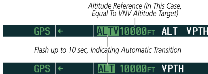
Figure 7-17 Automatic Mode Transitions During Altitude Capture
