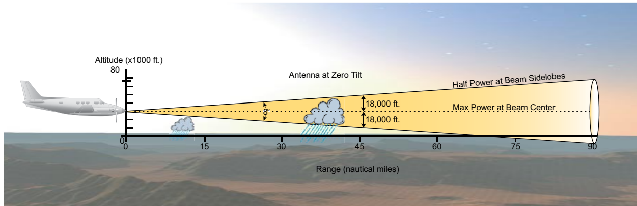
Figure 6-44 Radar Beam from a 12 inch Antenna
