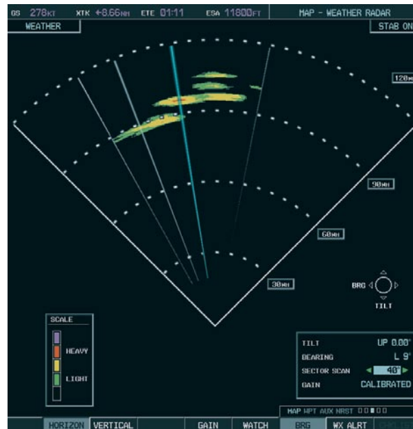
Figure 6-60 40° Sector Scan
