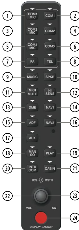
Figure 1-5 Audio Panel Controls (GMA 1347D-20)
