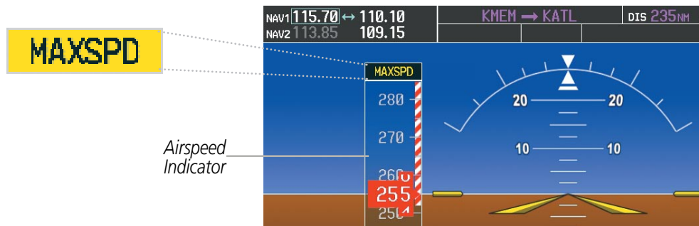
Figure 7-46 Overspeed Annunciation
