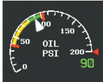
Figure 3-10 Oil Pressure Gauge
