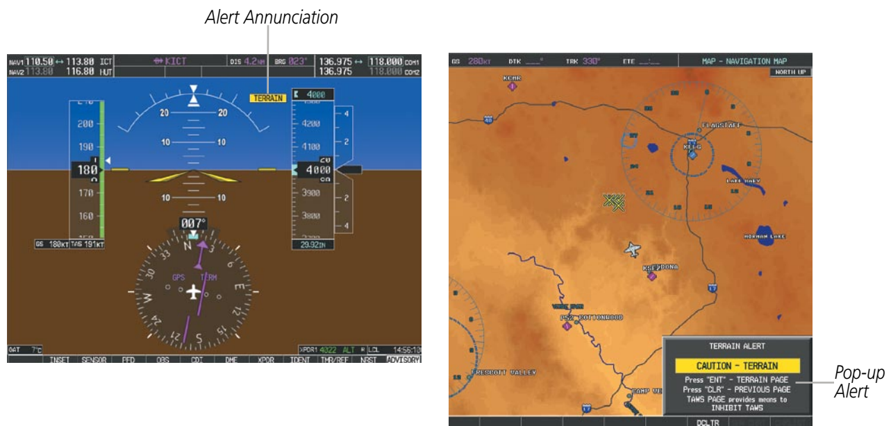
Figure 6-77 TAWS Alert Annunciations
