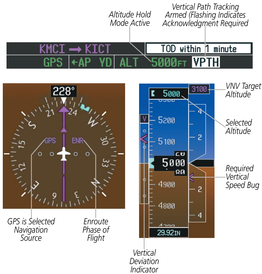
Figure 7-14 Vertical Path Capture
