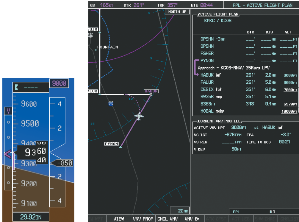
Figure 5-139 Descending Turn to the Initial Approach Fix (IAF)
