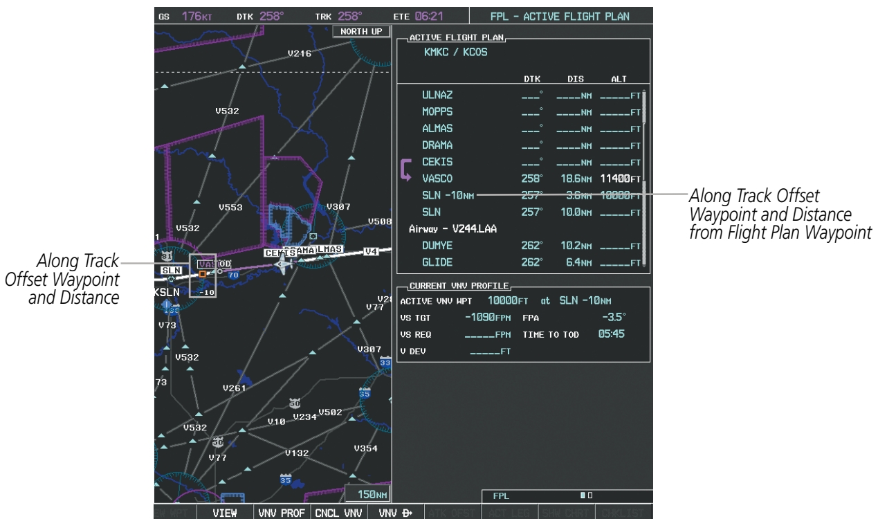
Figure 5-76 Along Track Offset
