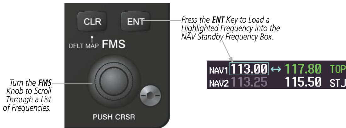
Figure 4-23 NAV Frequency Auto-Tuning from the MFD
