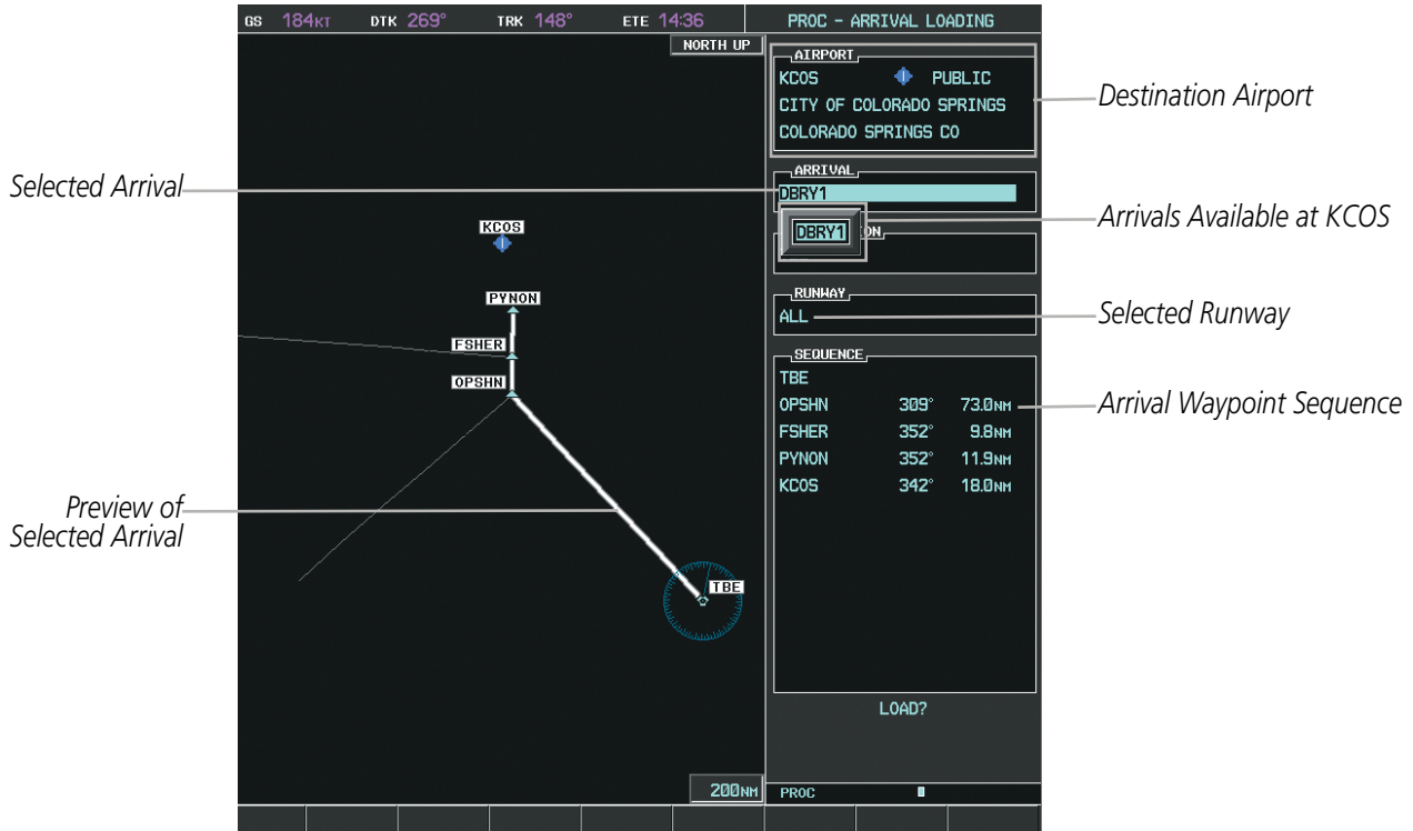
Figure 5-69 Arrival Loading Page - Selecting the Arrival
