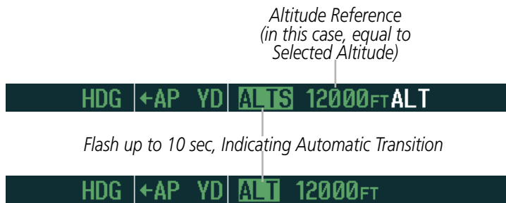
Figure 7-8 Automatic Mode Transitions During Altitude Capture
