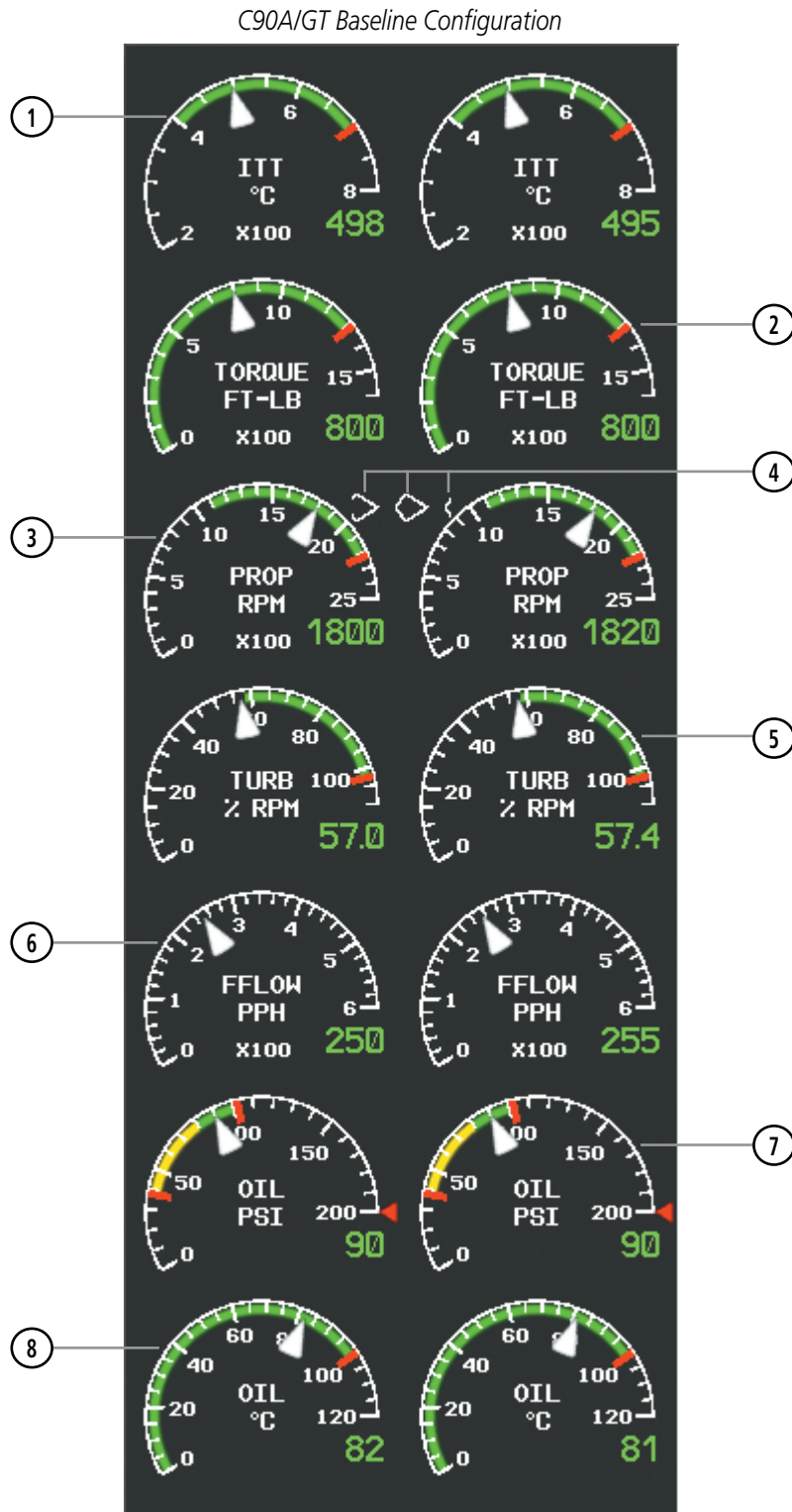
Figure 3-2 EIS Display
