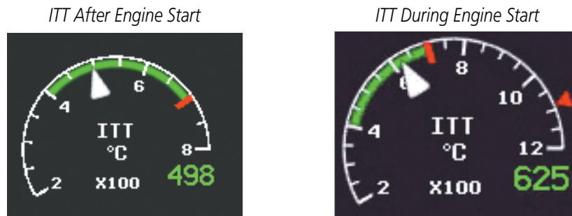
Figure 3-3 ITT Gauge
