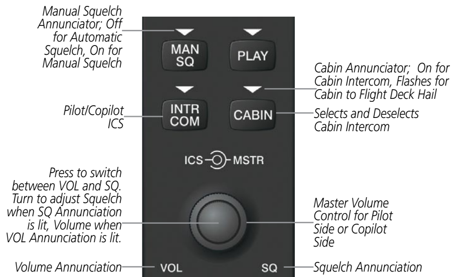
Figure 4-42 Intercom Controls
