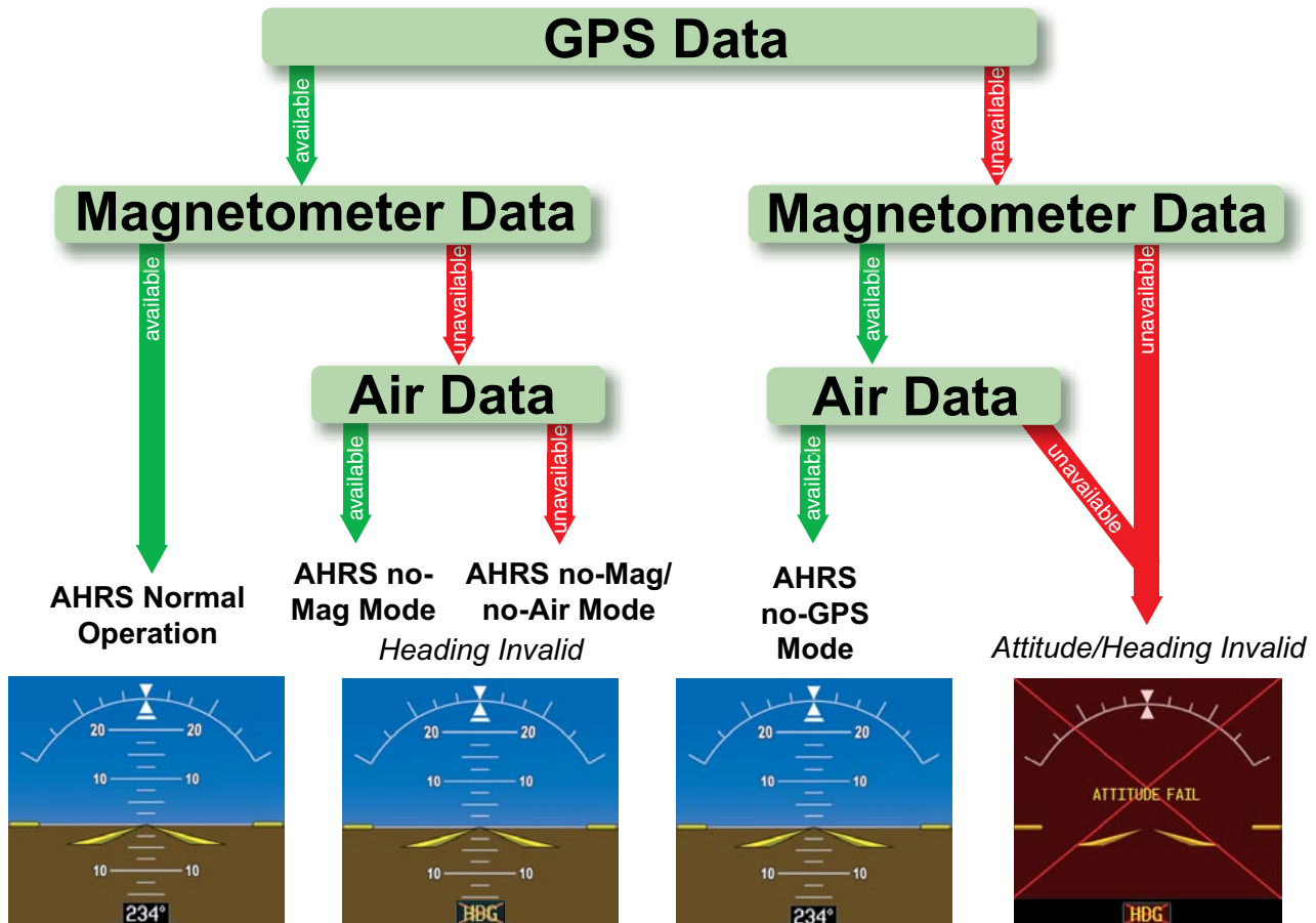
Figure 1-13 AHRS Operation
