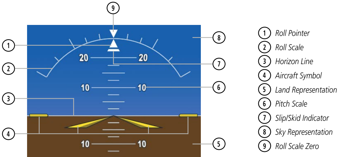
Figure 2-8 Attitude Indicator
