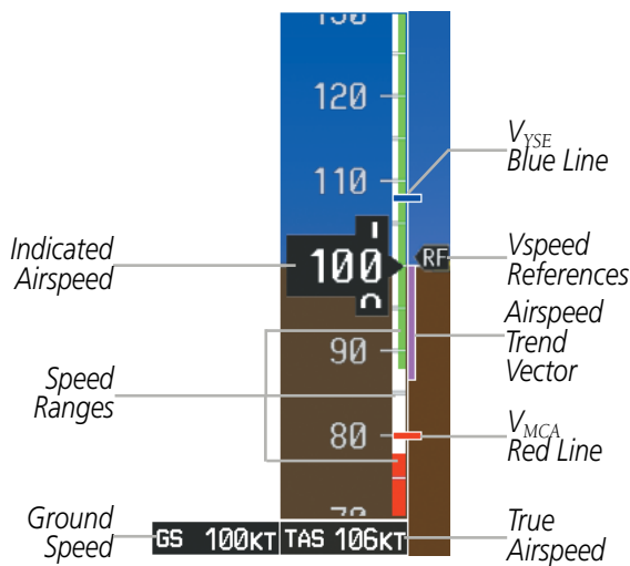
Figure 2-3 Airspeed Indicator
