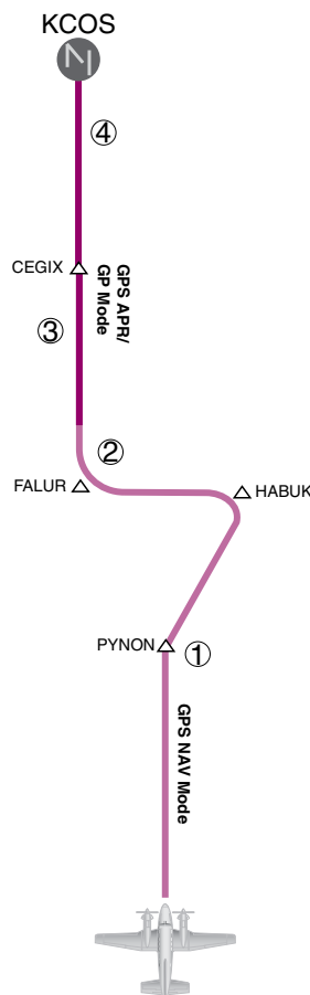
Figure 7-43 LPV Approach to KCOS
