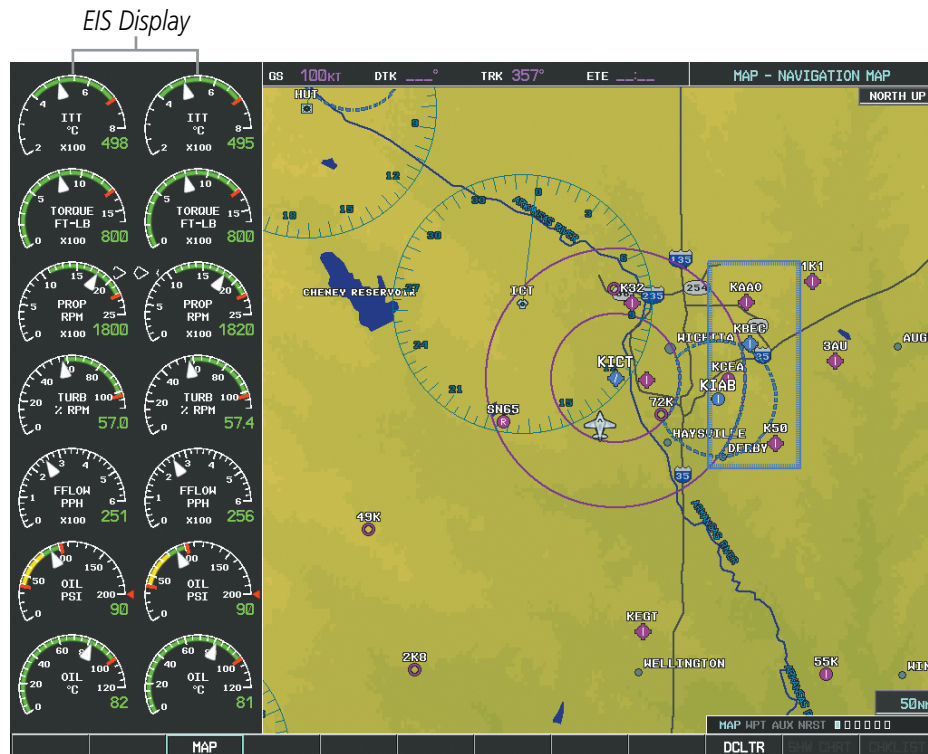
Figure 3-1 MFD (C90A/GT)
