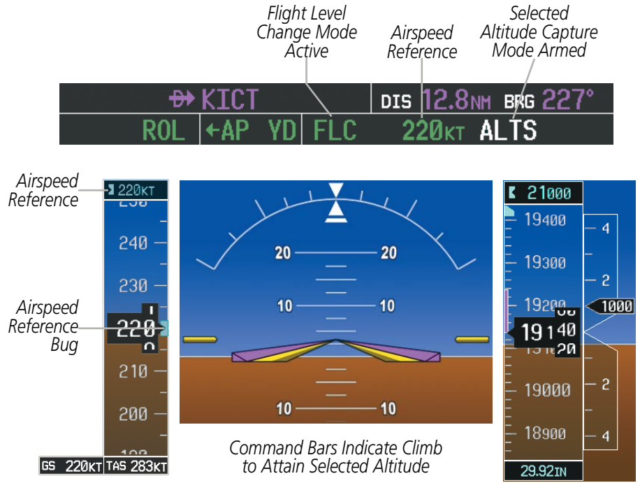
Figure 7-11 Flight Level Change Mode (IAS)
