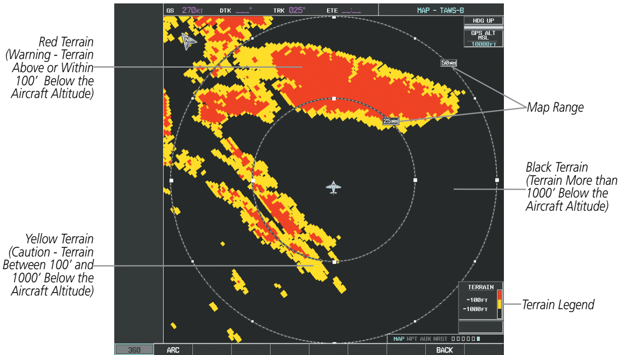
Figure 6-75 TAWS-B Page, 360° View
