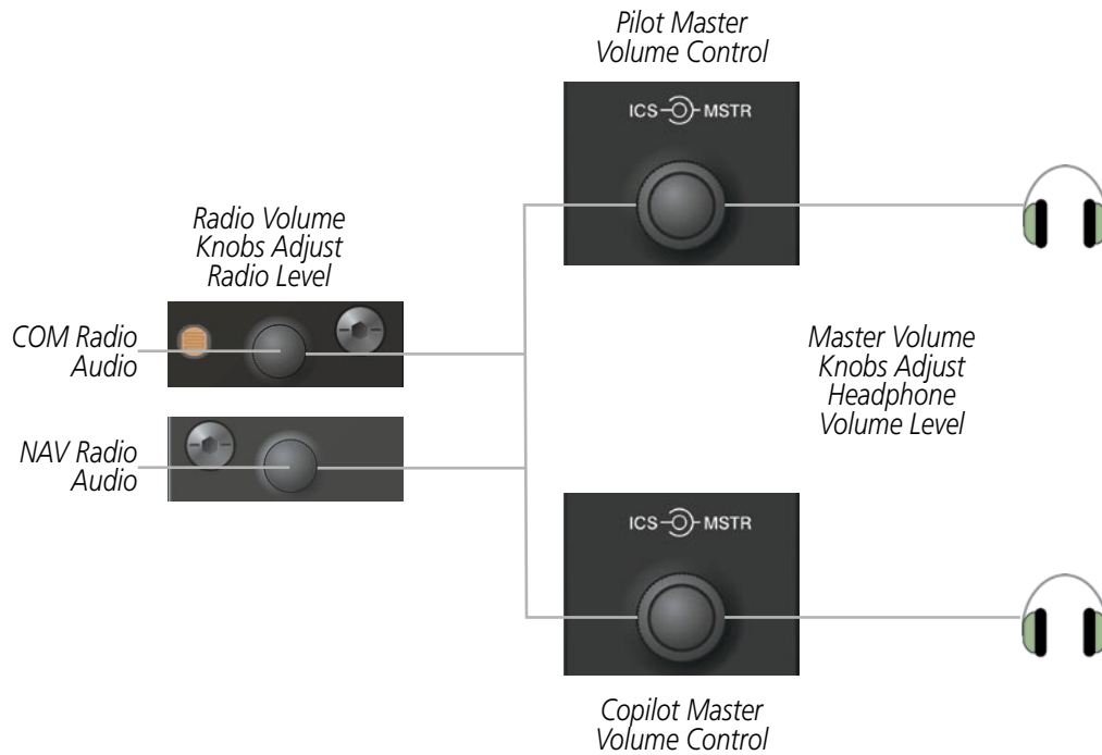
Figure 4-46 Radio and Headphone Volume Controls
