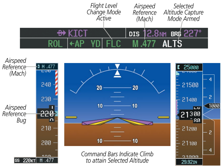
Figure 7-12 Flight Level Change Mode (Mach)
