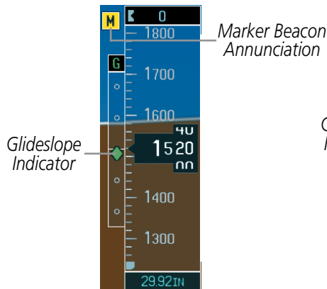
Figure 2-16 Glideslope Indicator
