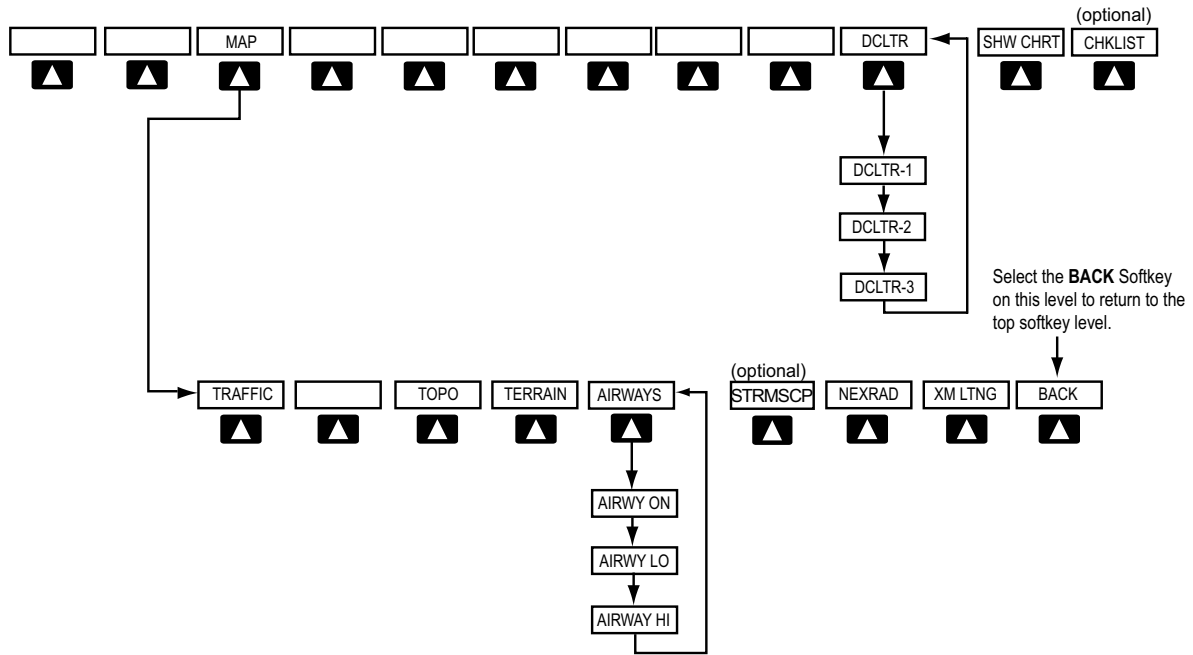
Figure 1-21 MFD Softkeys
