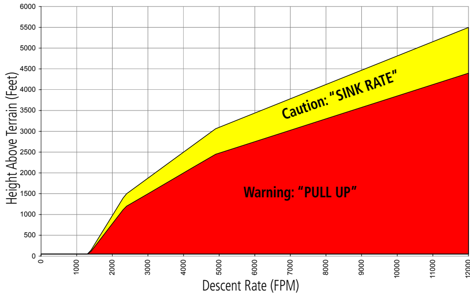
Figure 6-79 Excessive Descent Rate Alert Criteria
