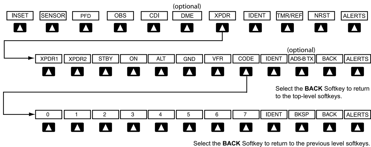
Figure 1-20 XPDR Softkeys
