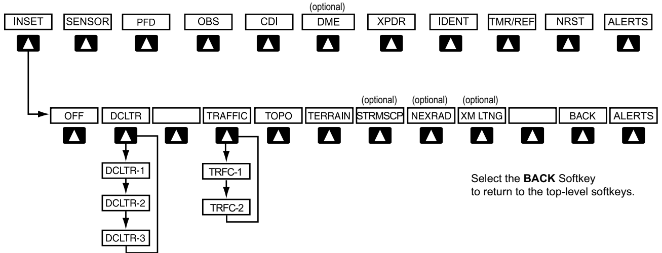
Figure 1-17 INSET Softkeys
