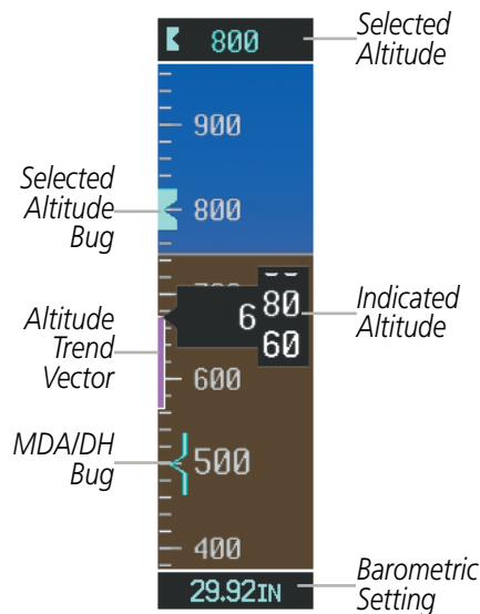
Figure 2-11 Altimeter
