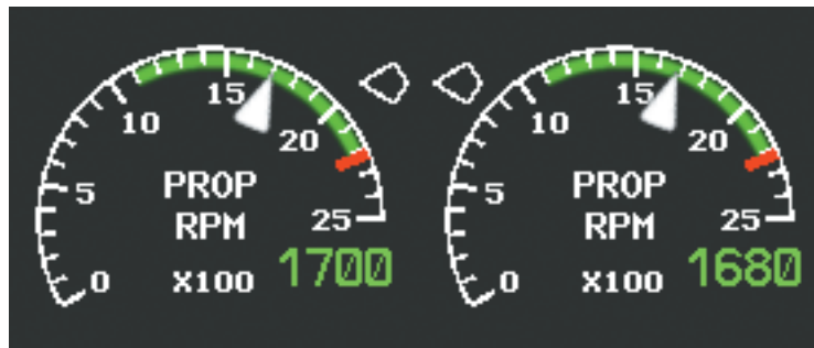
Figure 3-6 Tachometer with Propellers Out of Sync (less than 50 rpm)
