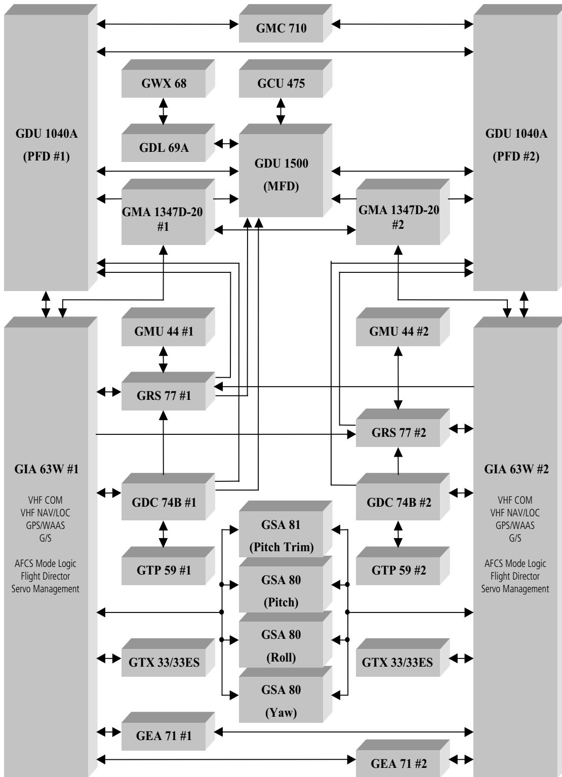
Figure 1-1 G1000 System (LRU Configuration)
