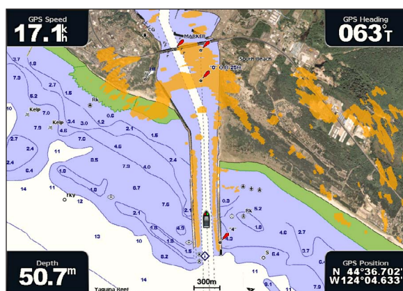
Radar Overlay on the Navigation Chart
