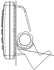
Figure 1 Pull gimbal bracket down until cam lobe contacts surface.
