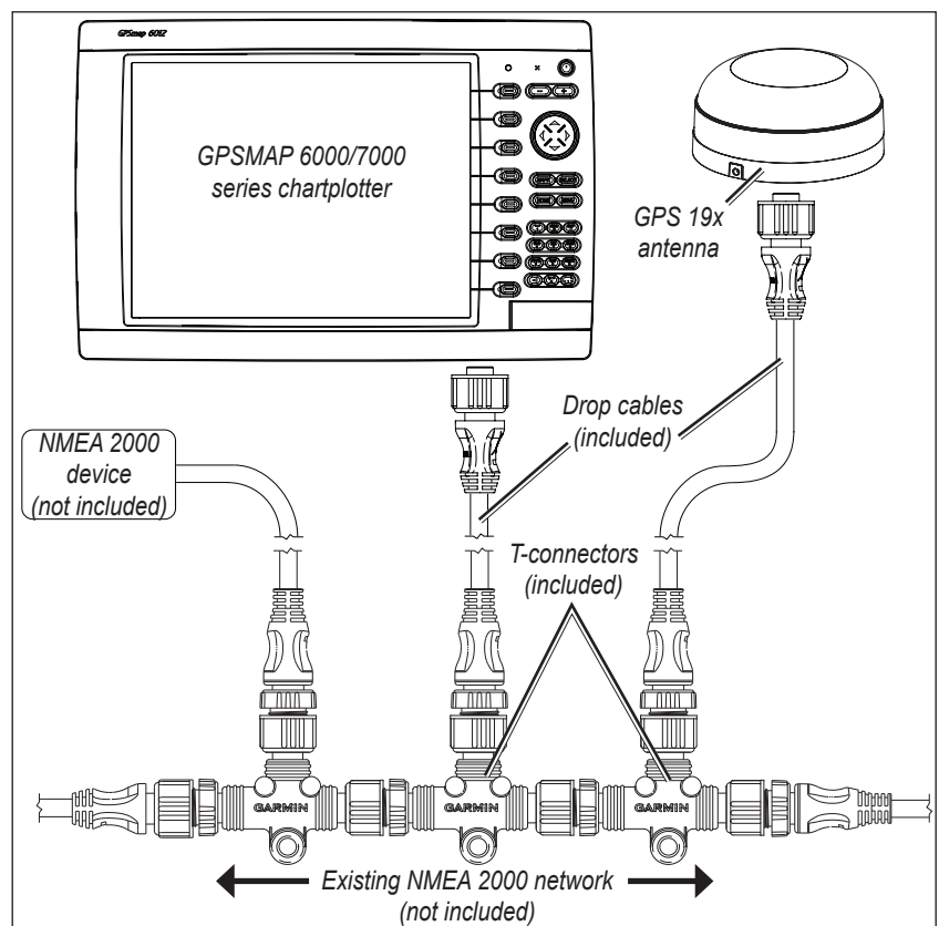
Connecting a GPSMAP 6000/7000 Series Chartplotter and a GPS 19x Antenna to an Existing NMEA 2000 Network
