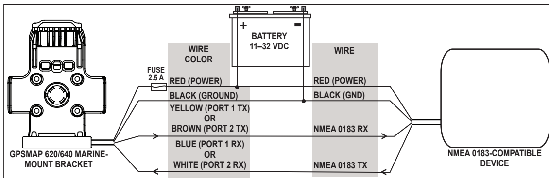
Wiring the GPSMAP 620/640 Marine-Mount Bracket to a NMEA 0183-compatible Device
