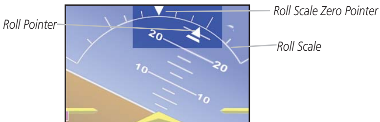
G600 Attitude Indicator with a Sky Pointer Configuration in a Left Turn
