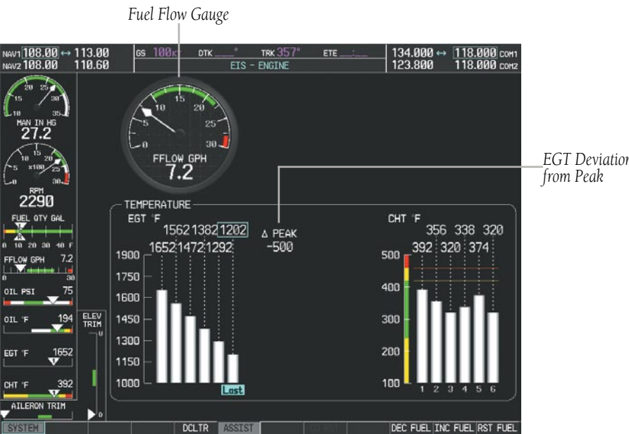
Engine Leaning Assist Mode (Cessna 350)
