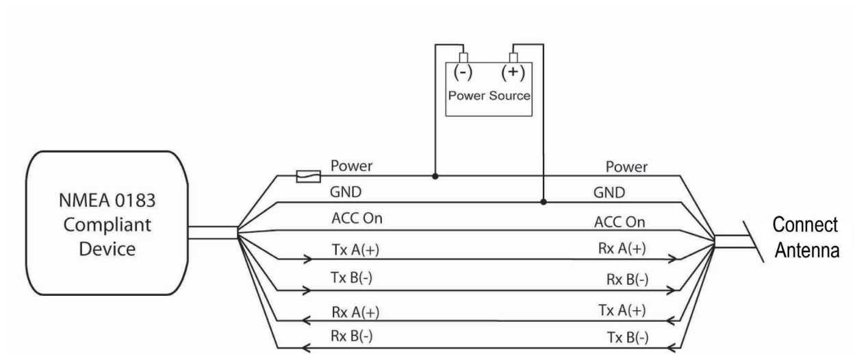
Figure 3a. GPS 19x NMEA 0183 HVS Wired for Two-Way Communication
